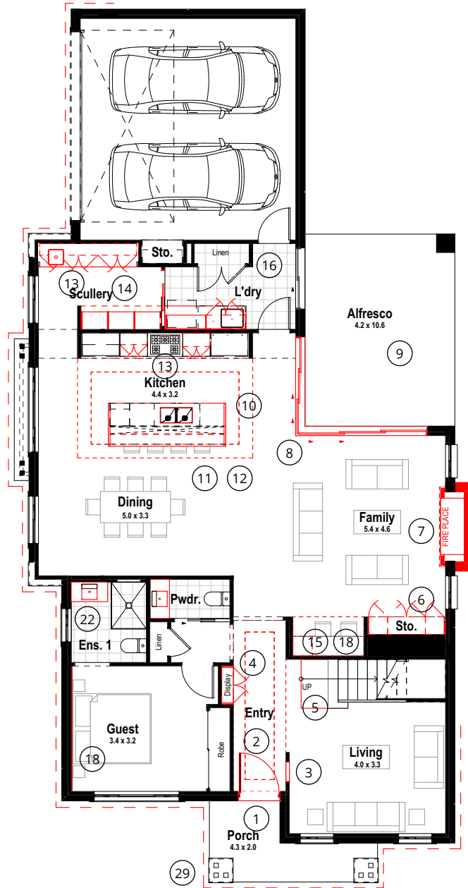
Ground Floor
