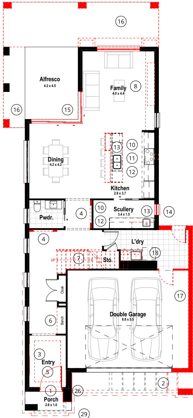
Ground Floor
